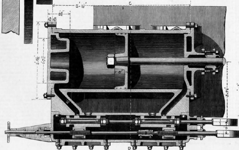
SECTIONAL PLAN OF CYLINDER AT A.B.
