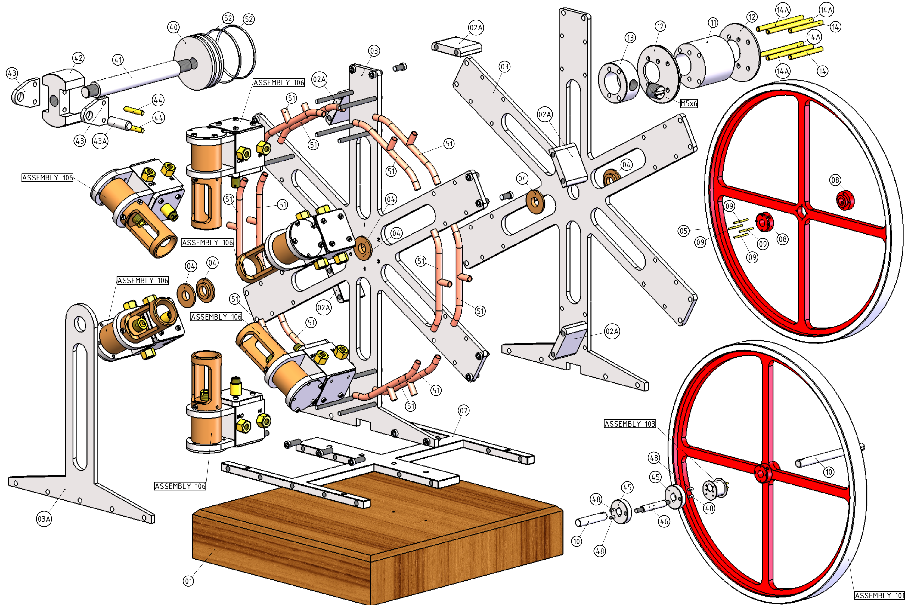
TITLE SIX CYLINDER RADIAL STEAM ENGINE WITH SLIDE VALVES ASSEMBLIES AND PARTS
