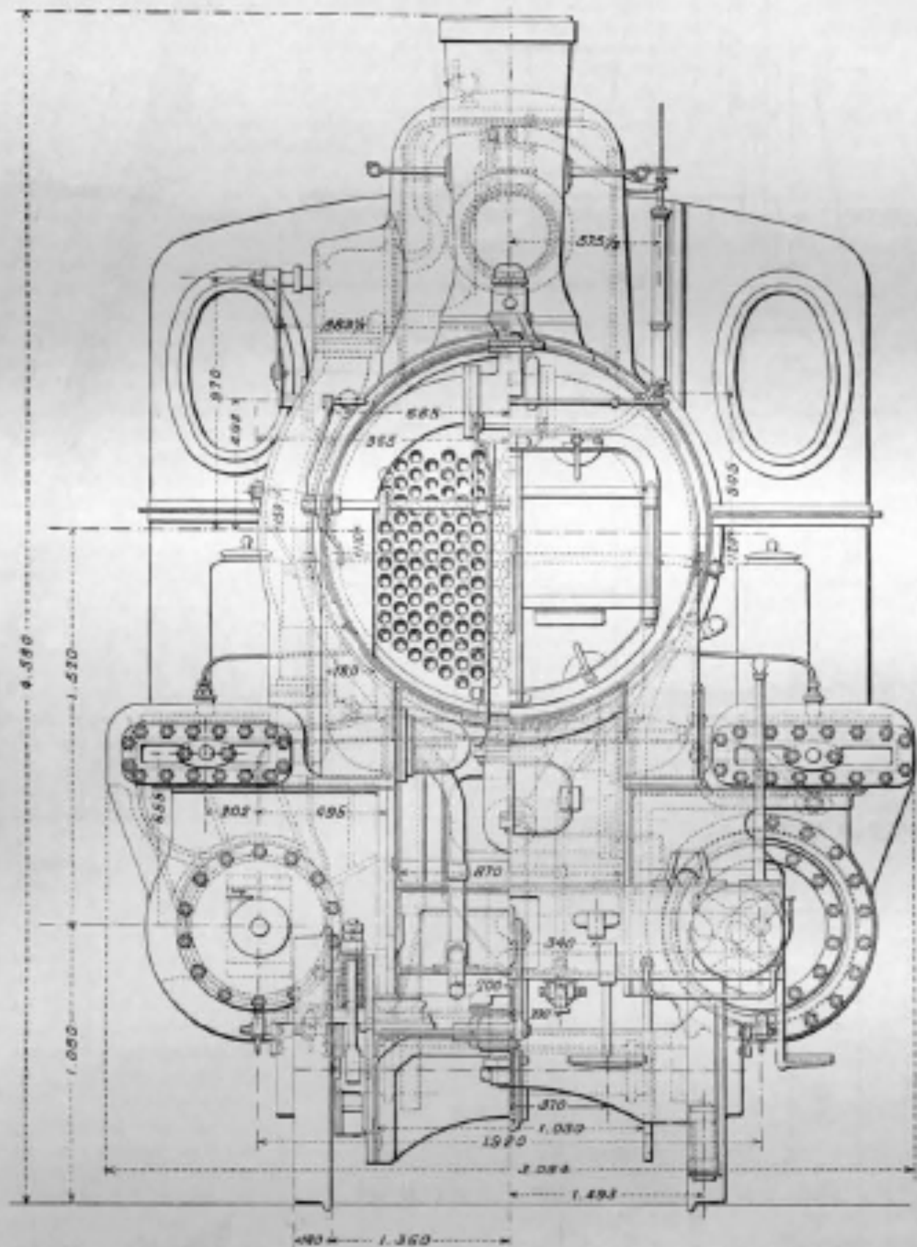
COMPOUND AUSTRIAN LOCOMOTIVE
