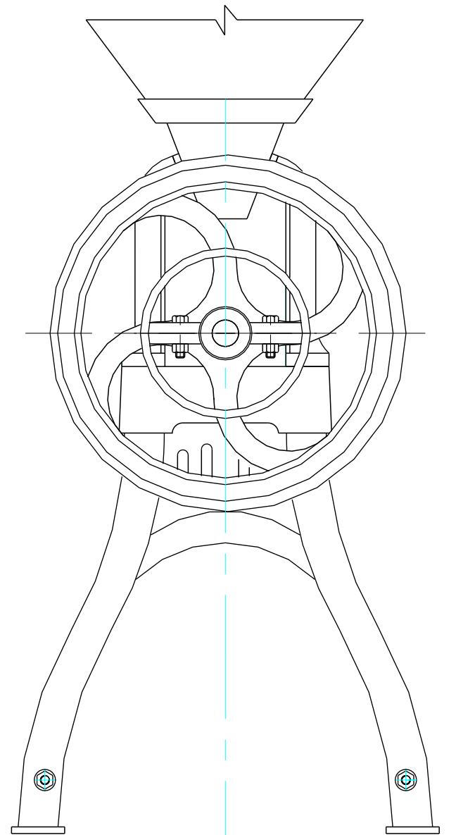
PULLEY END VIEW
