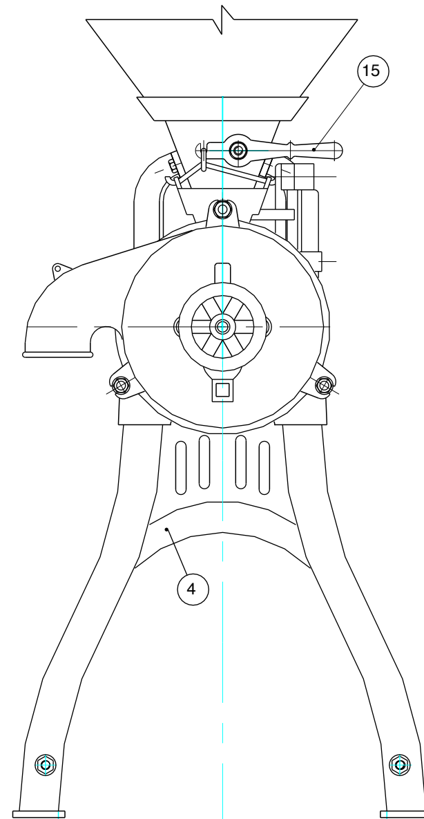
GRINDING END VIEW
