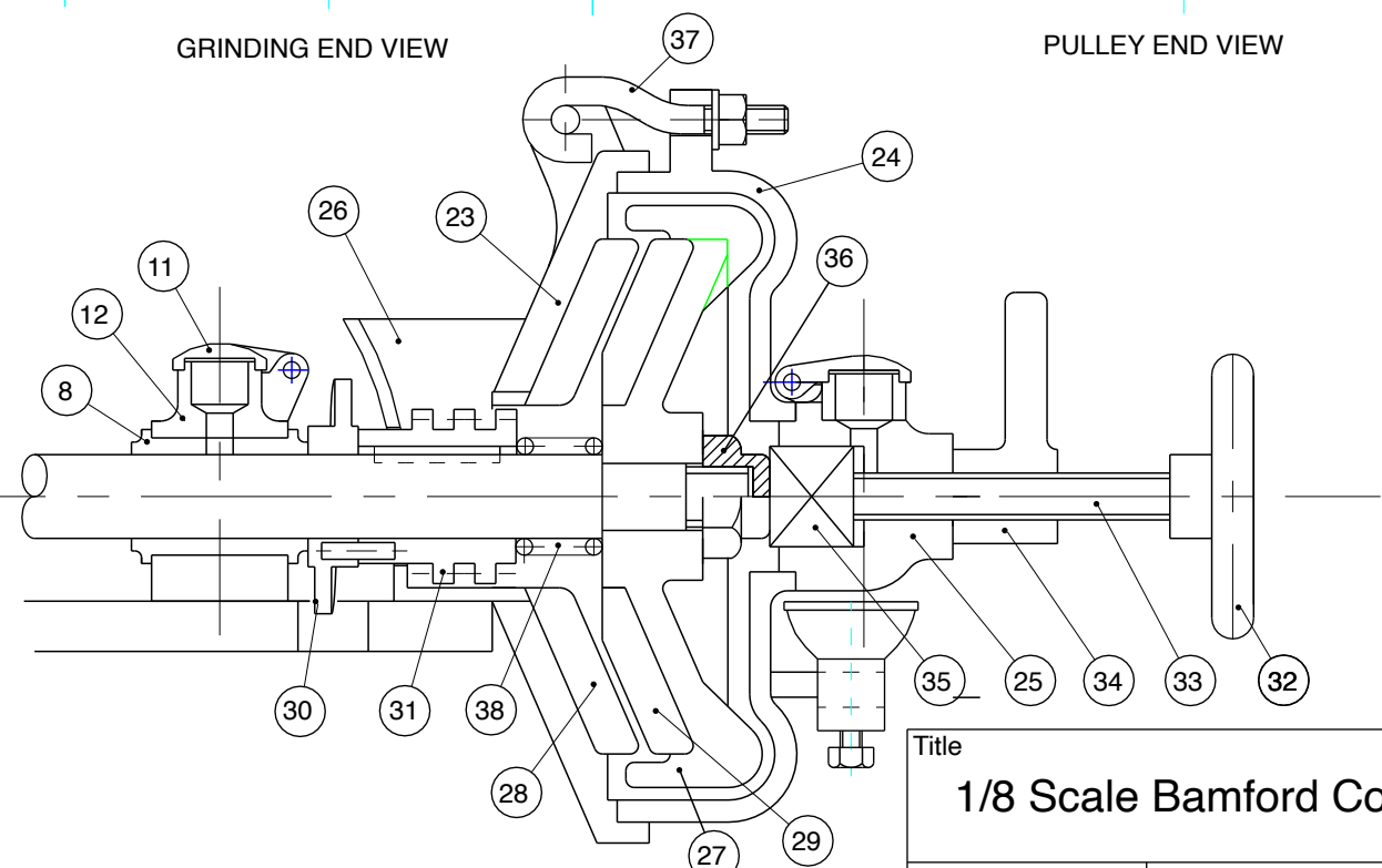
GRINDER HEAD SECTION 2X FULL SIZE
