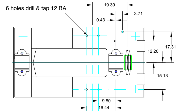
Bedplate Drilling Details
