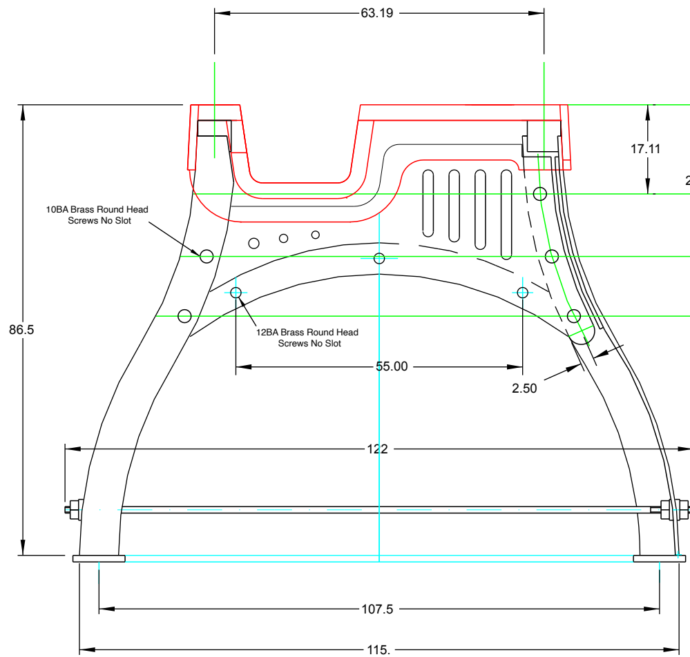
ELEVATION (half section)
