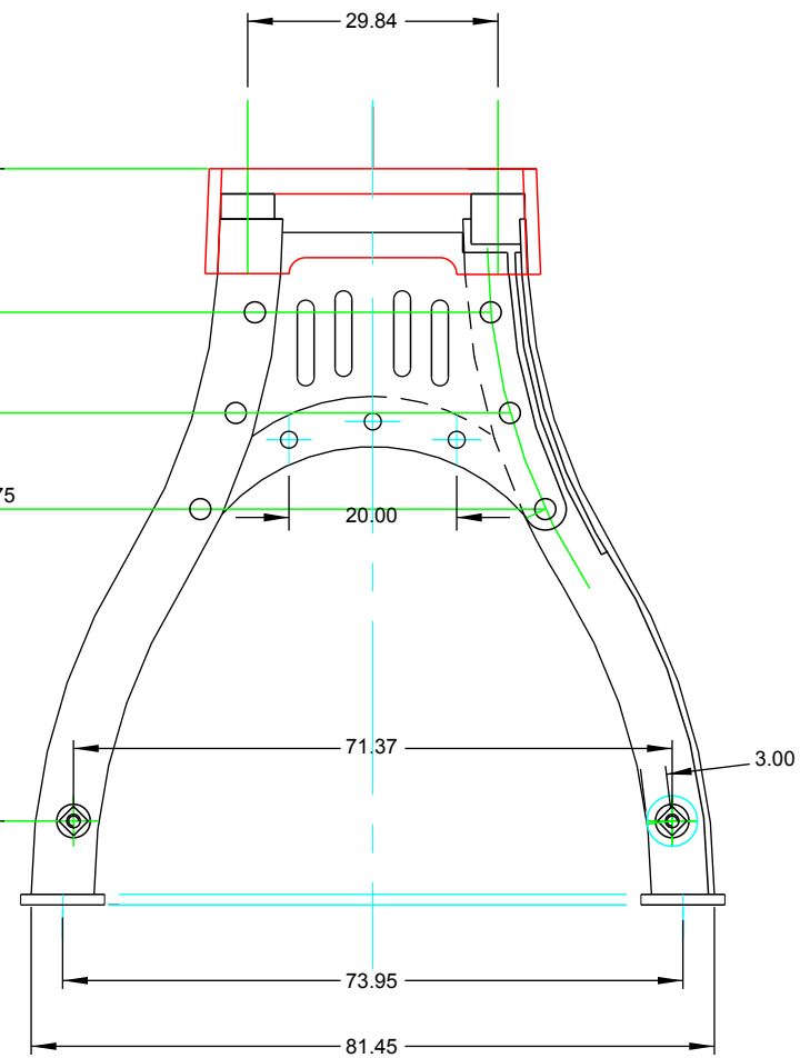
END ELEVATION (half section)
