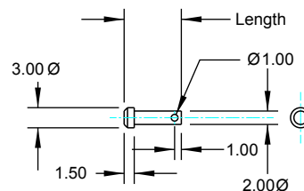
(44) Pins - Mild Steel 1 - Length 10.00 2 - Length 8.00
