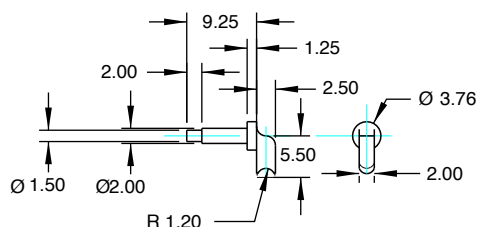
(22) LOCKING LATCH - Mild Steel
