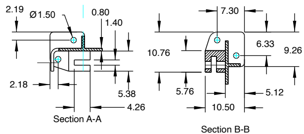
(18) SHAKER SUPPORT BRACKET - Brass
