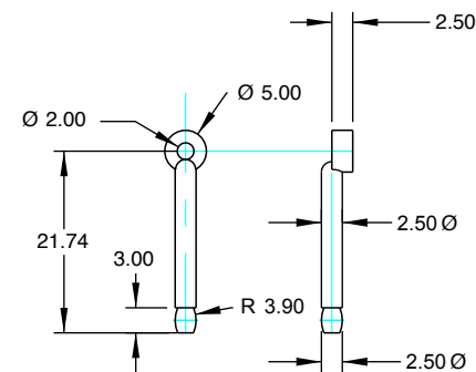
(19) ROCKING ARM - Mild Steel
