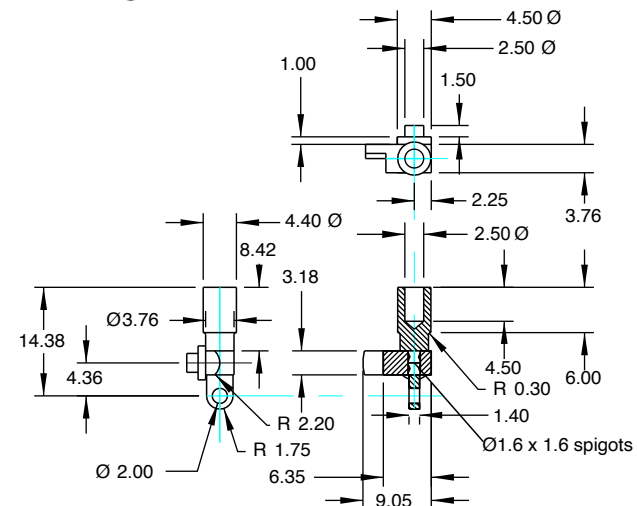
(20) ROCKING BLOCK - Brass
