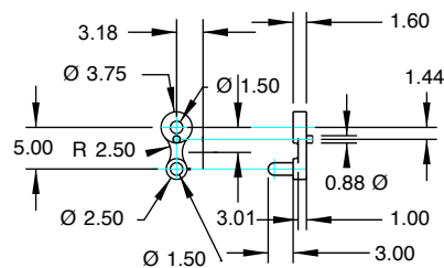
(21) LOCKING LEVER - Brass Steel Pin
