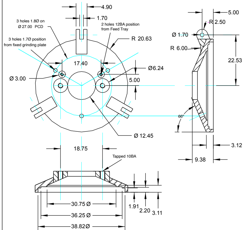
23 FIXED HOUSING - Brass
