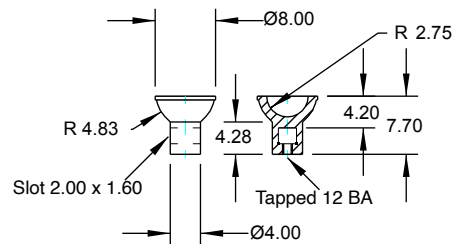
41 OIL CATCH POT - Brass
