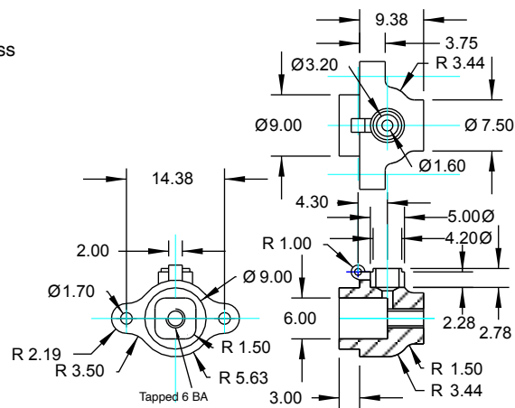
25 PRESSURE BLOCK - Brass
