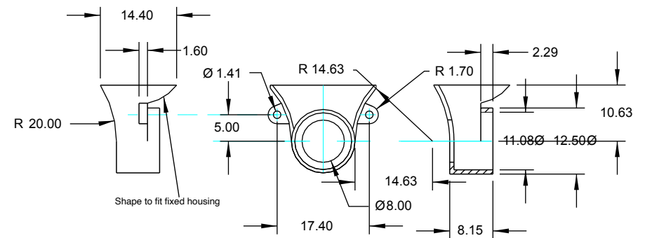
26 FEED SHUTE - 22 swg Brass
