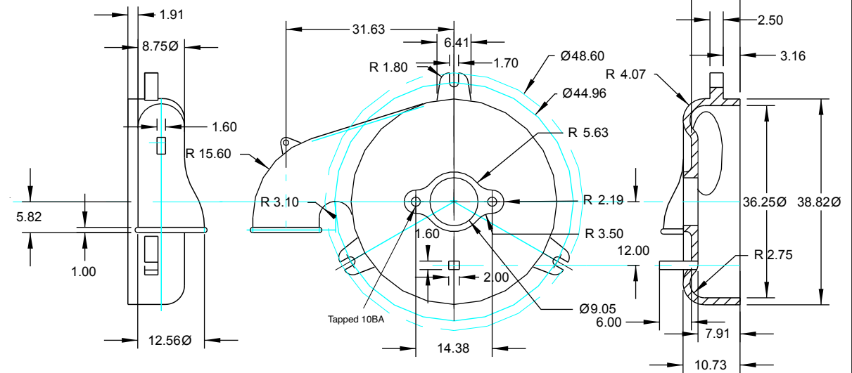
24 REMOVABLE HOUSING - Brass
