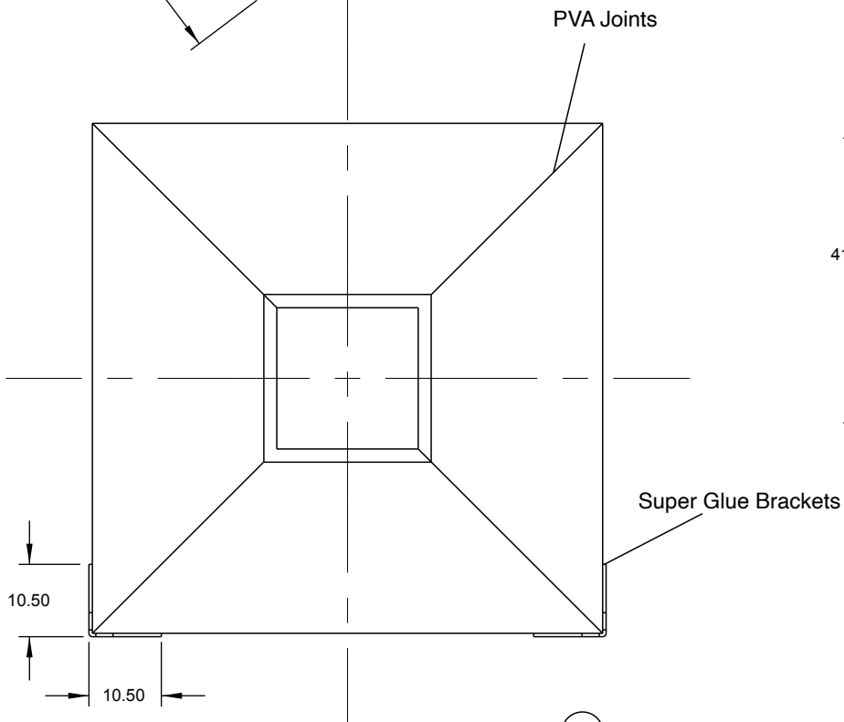
43 CORN FEED BOX - 1.5 mm Plywood Brackets - 0.5mm Brass
