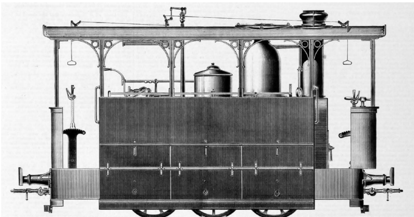
FIG 36. SIDE ELEVATION
