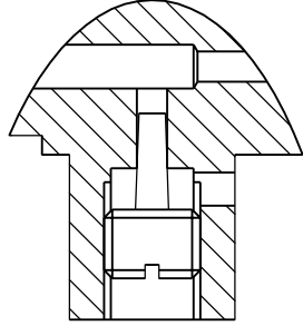
AIR BLEED ACROSS JET
