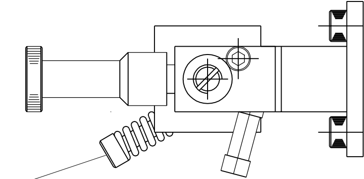
IDLE THROTTLE STOP
