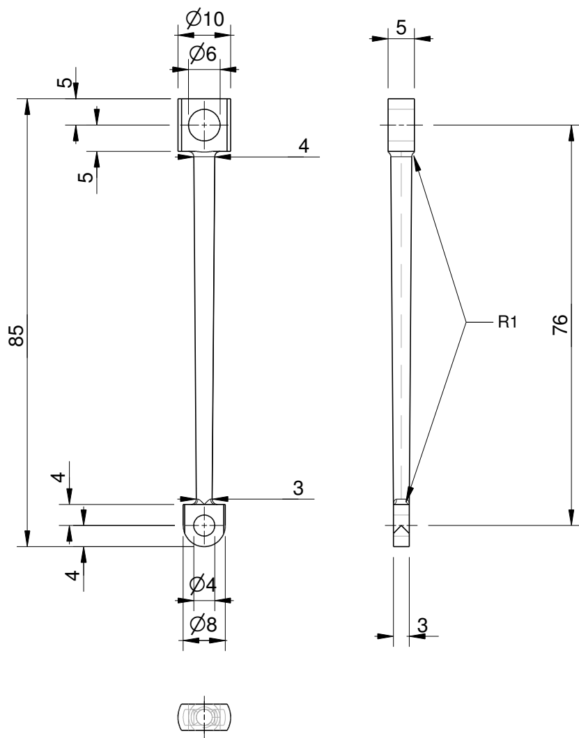
Conrod Aluminium Scale 1:1 1 req'd
