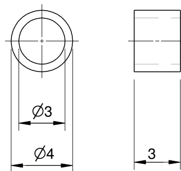
Small End bearing Bronze Scale 1:1 1 Req'd
