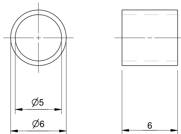
Big End Bearing Bronze Scale 4:1 1 Req'd
