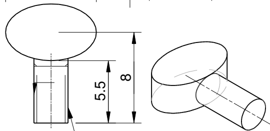
Burner Thumb Screw
