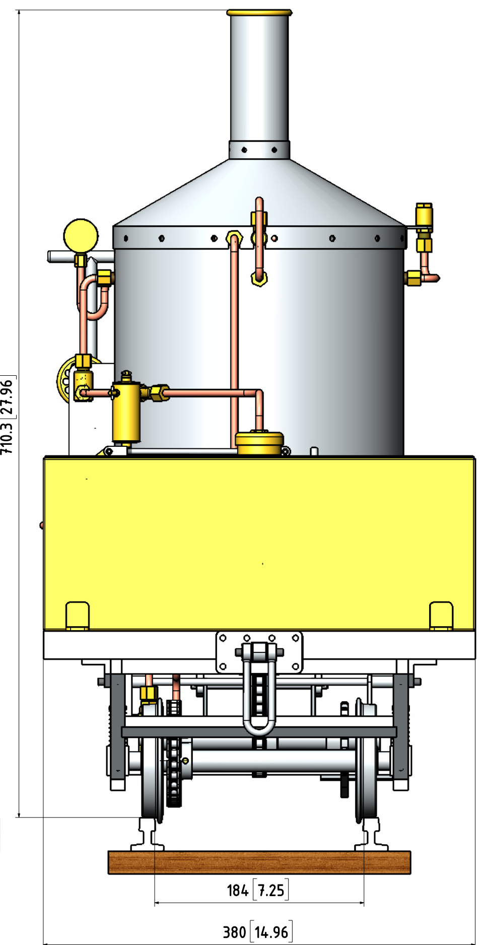
FRONT VIEW
