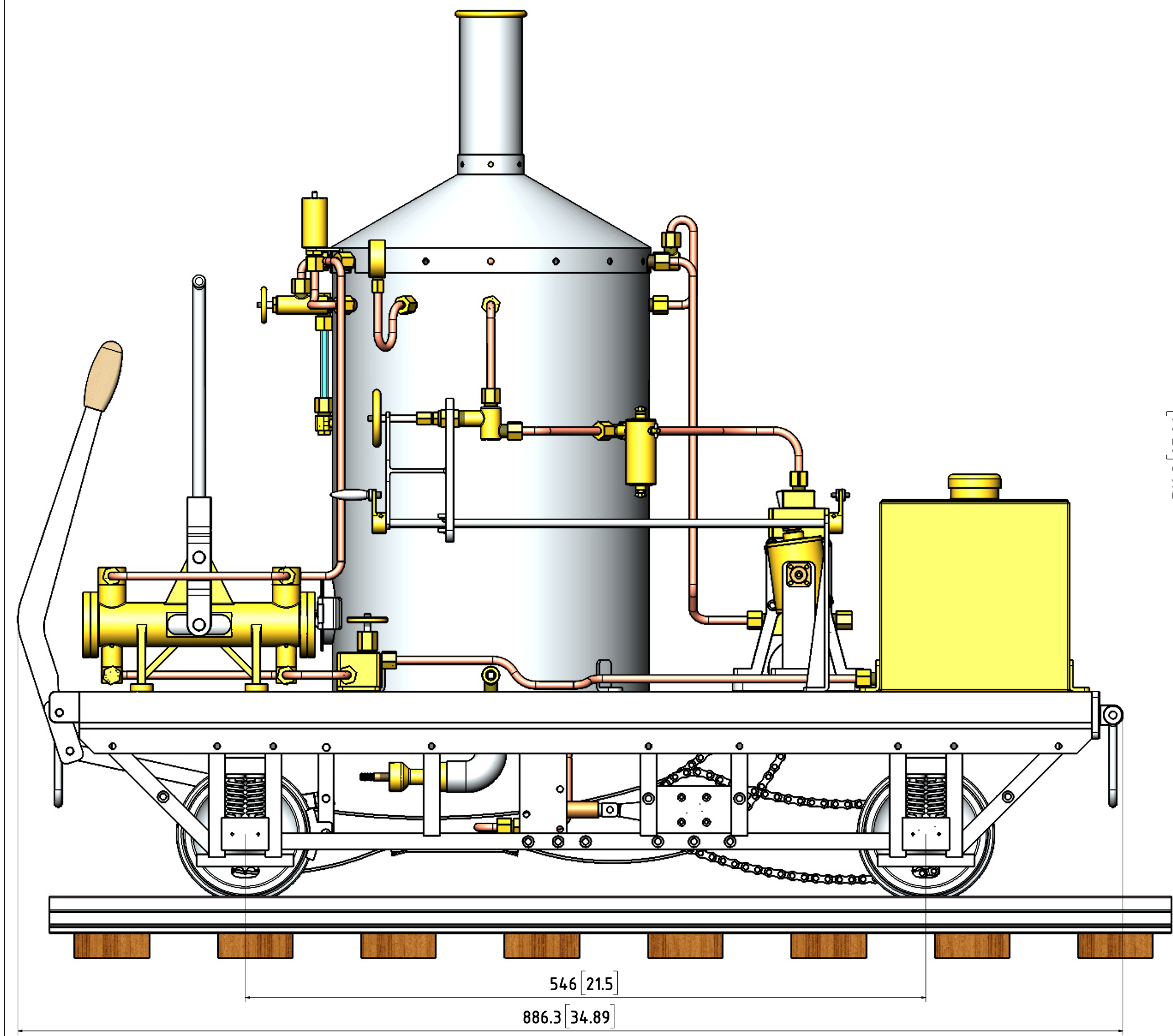
RIGHTHAND VIEW
