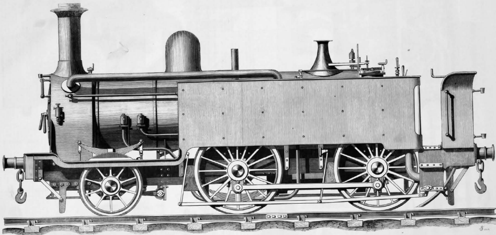
NARROW-GAUGE LOCOMOTIVE, METROPOLITAN SYSTEM, GREAT WESTERN RAILWAY.
