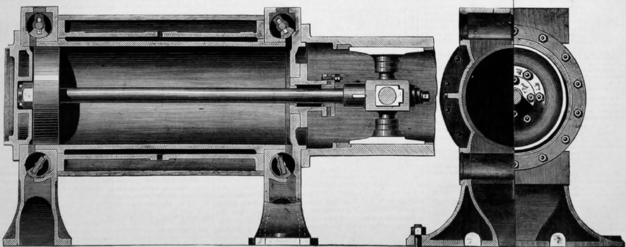
TRANSVERSE SECTION
