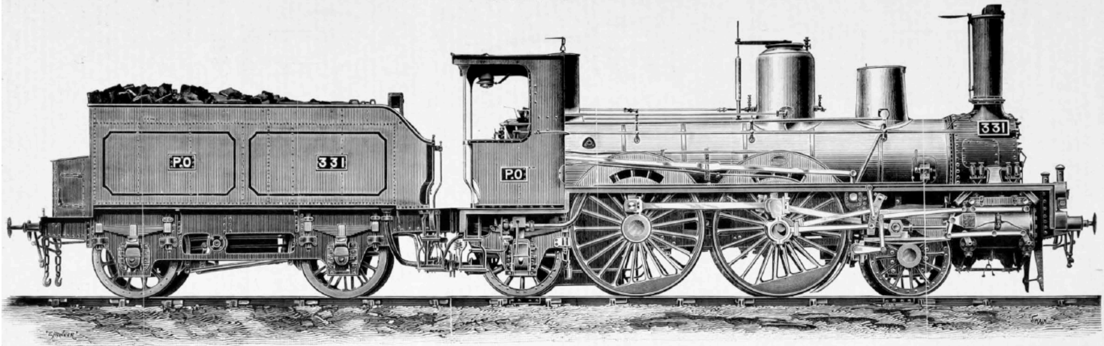
LOCOMOTIVE ENGINE WITH CORLISS VALVES, PARIS AND ORLEANS RAILWAY M. E. POLONCEAU, ENGINEER
