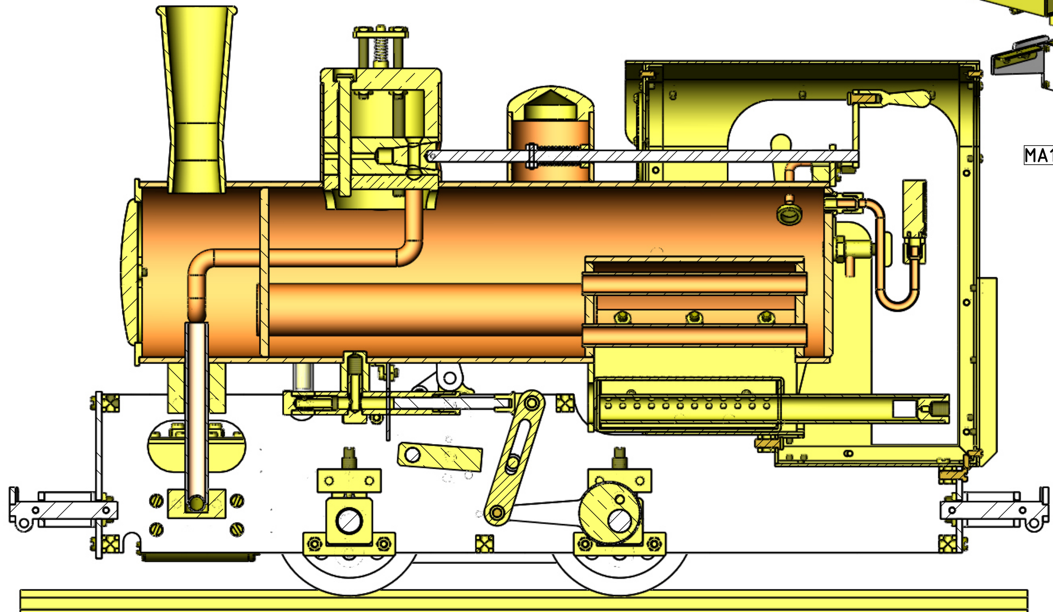
SECTION ON CENTRELINE
