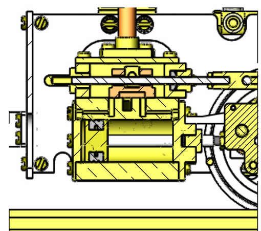
SECTION ON CYLINDER
