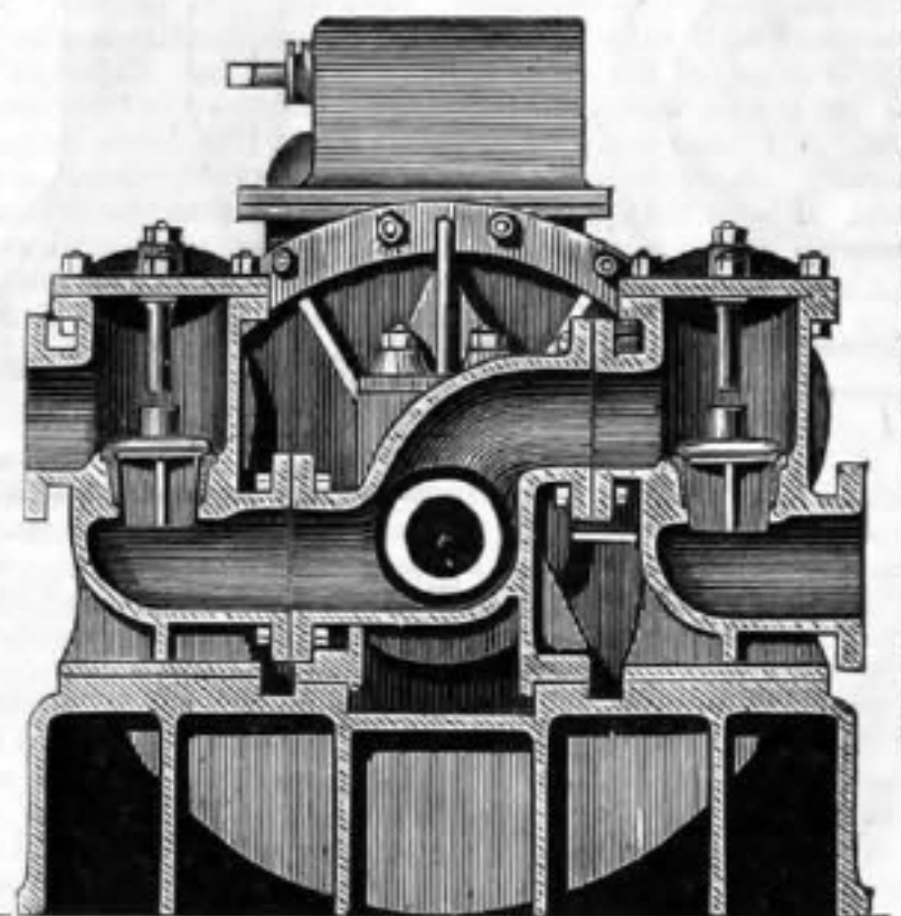
TRANSVERSE SECTION
