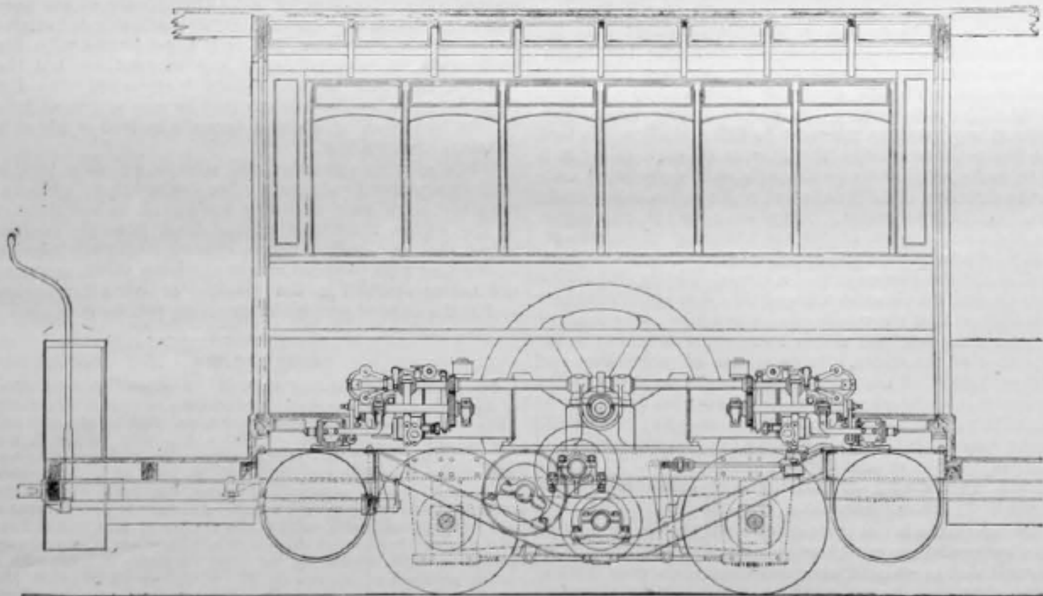
GAS MOTOR PROPELLED TRAM CAR-LONGITUDINAL SECTION
