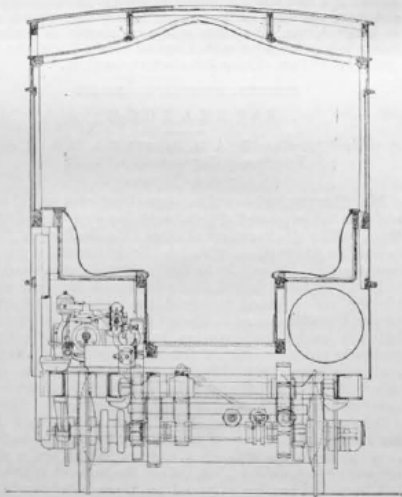
TRANSVERSE SECTION.
