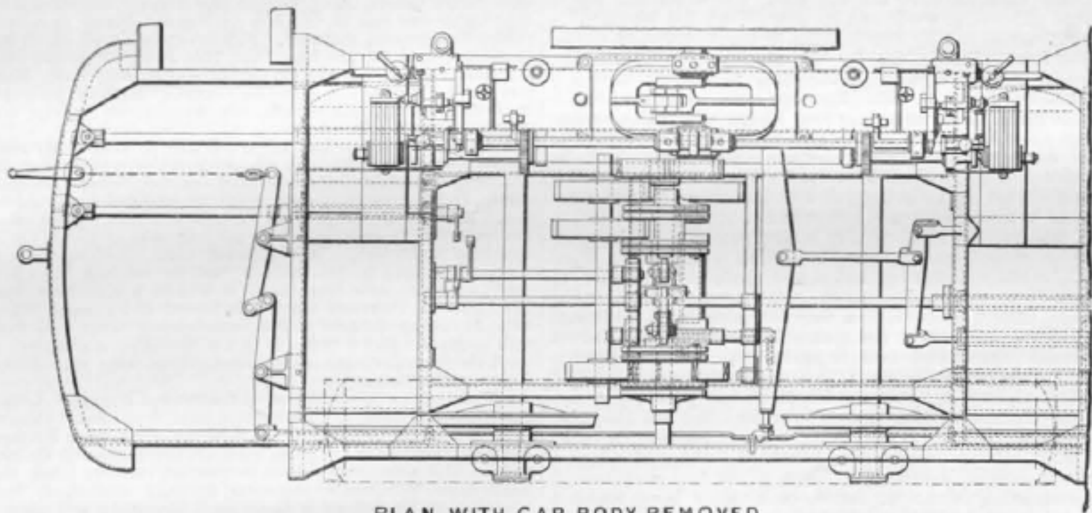
PLAN. WITH CAR BODY REMOVED.
