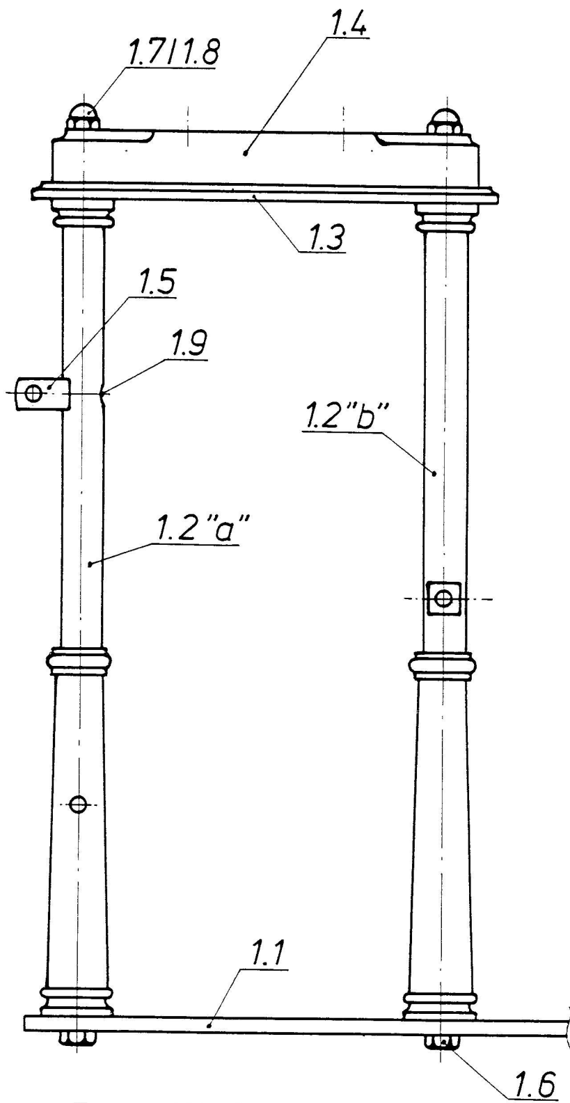
Frame Work
