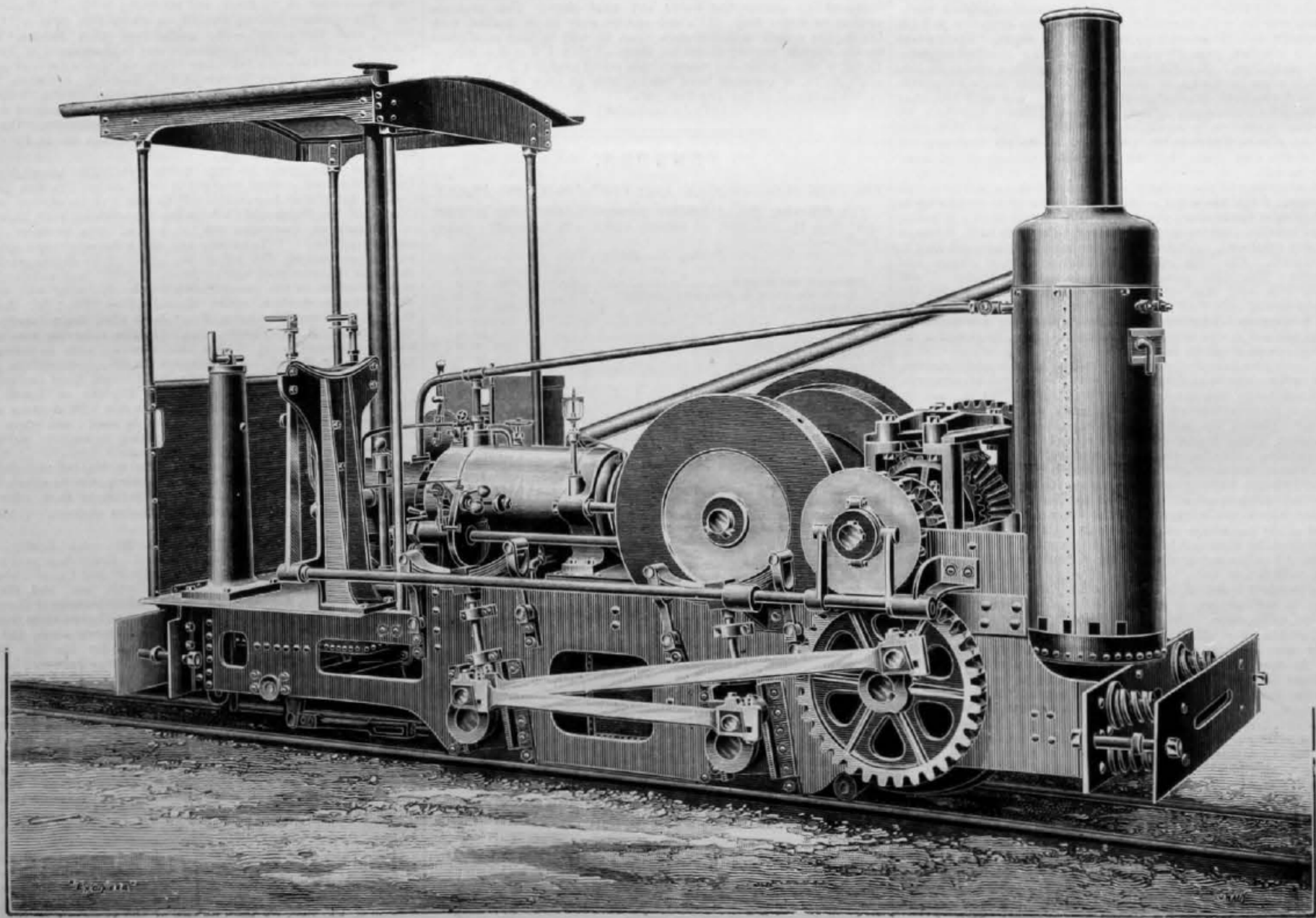
NARROW GAUGE LOCOMOTIVE
