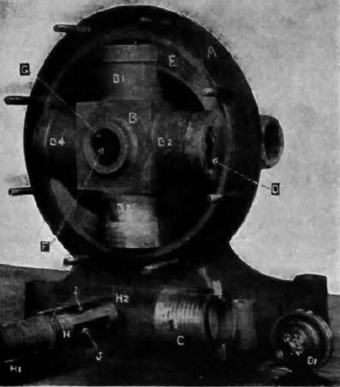
Fig. 1—CRANKLESS ENGINE
