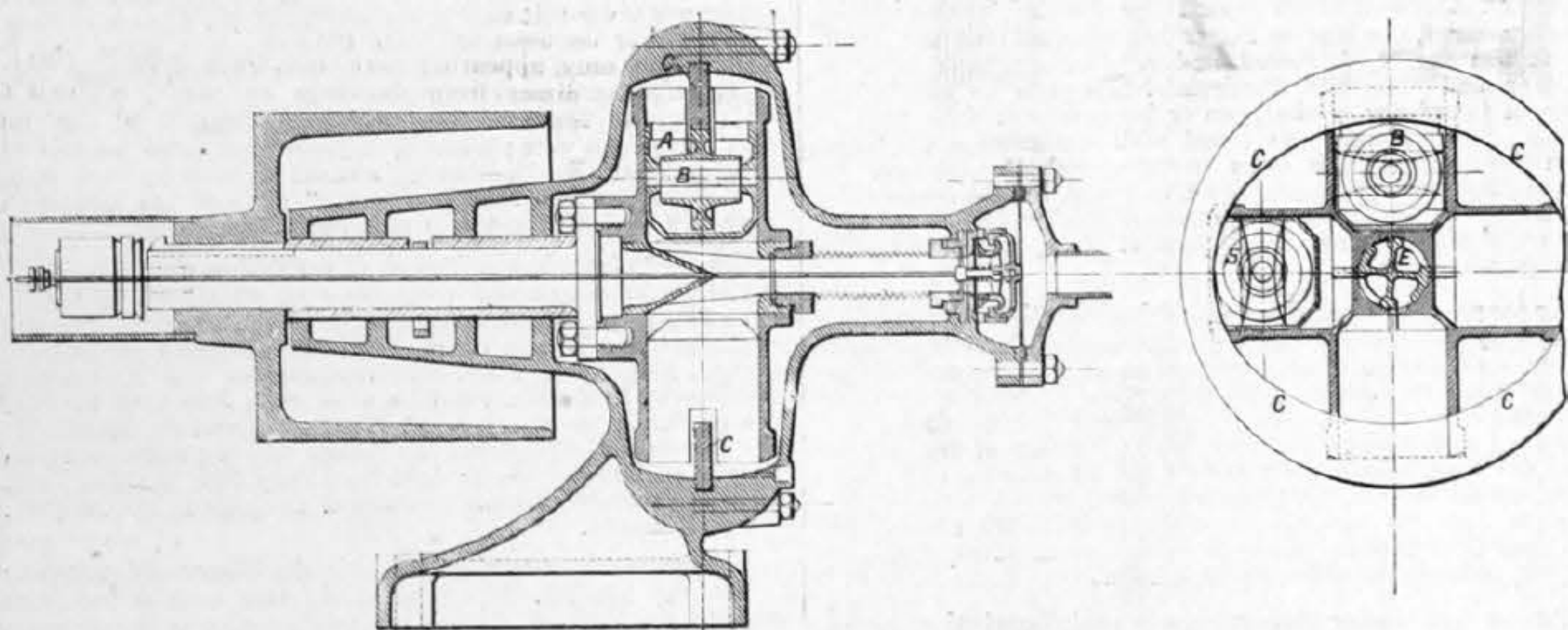
Fig. 2—CRANKLESS ENGINE—SECTION
