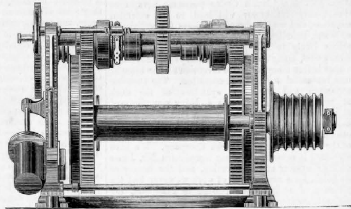
SIDE ELEVATION.
