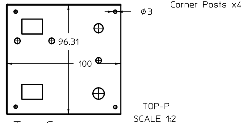
Top Cover
