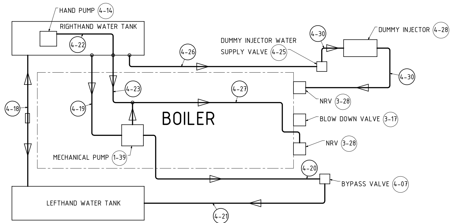
WATER SUPPLY PIPING DIAGRAM
