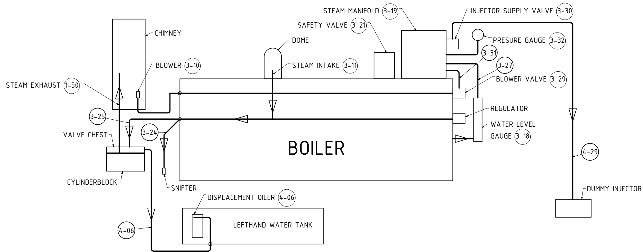
STEAM SUPPLY PIPING DIAGRAM
