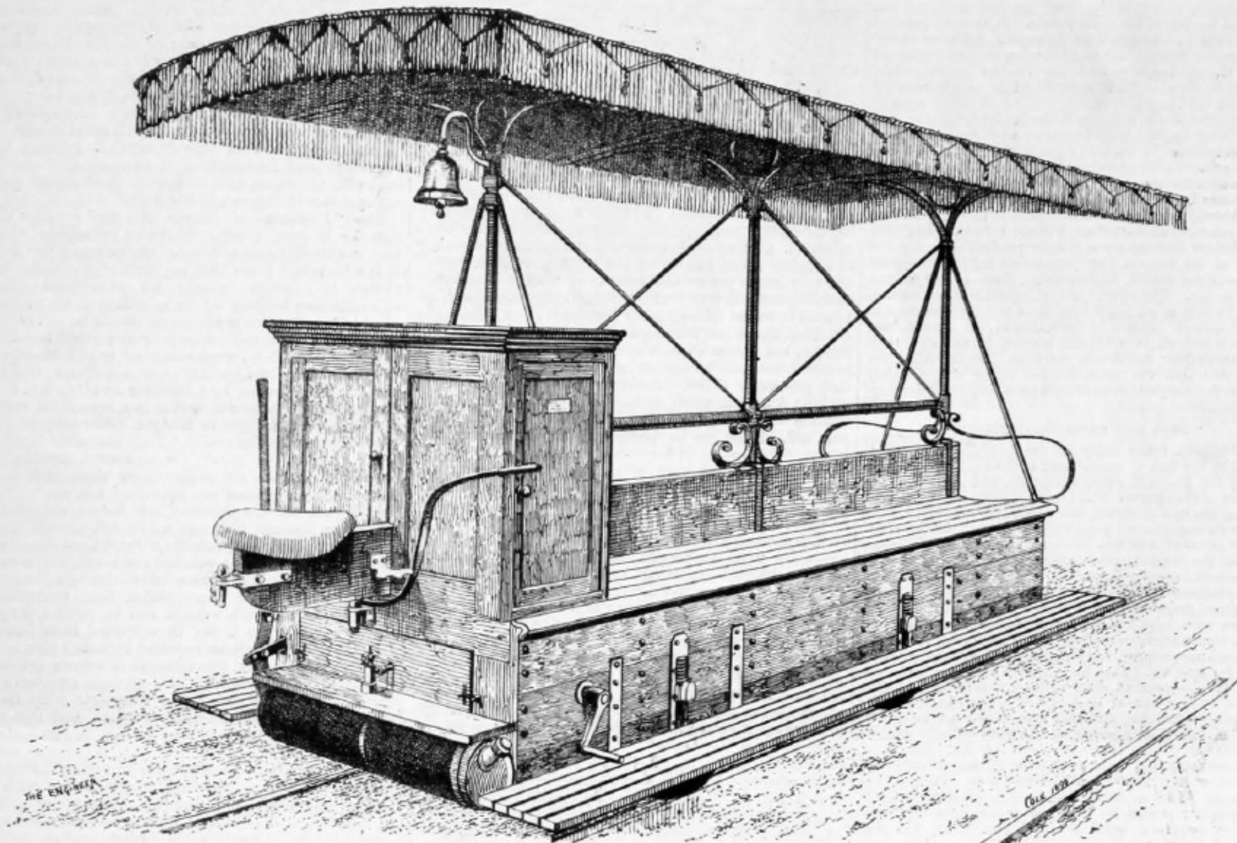
Fig. 1—PERSPECTIVE VIEW OF SELF-PROPELLED CAR FROM MOTOR END
