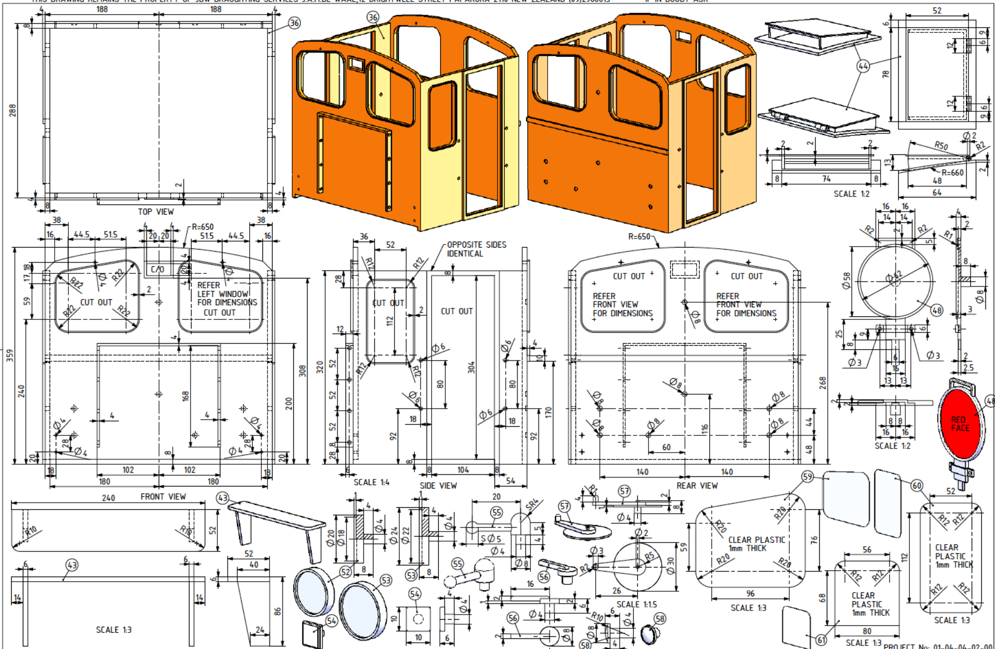
NARROW GAUGE DIESEL HYDRAULIC SHUNTING LOCO "THE KOF"
