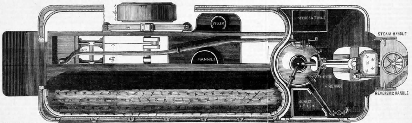
SECTIONAL PLAN
