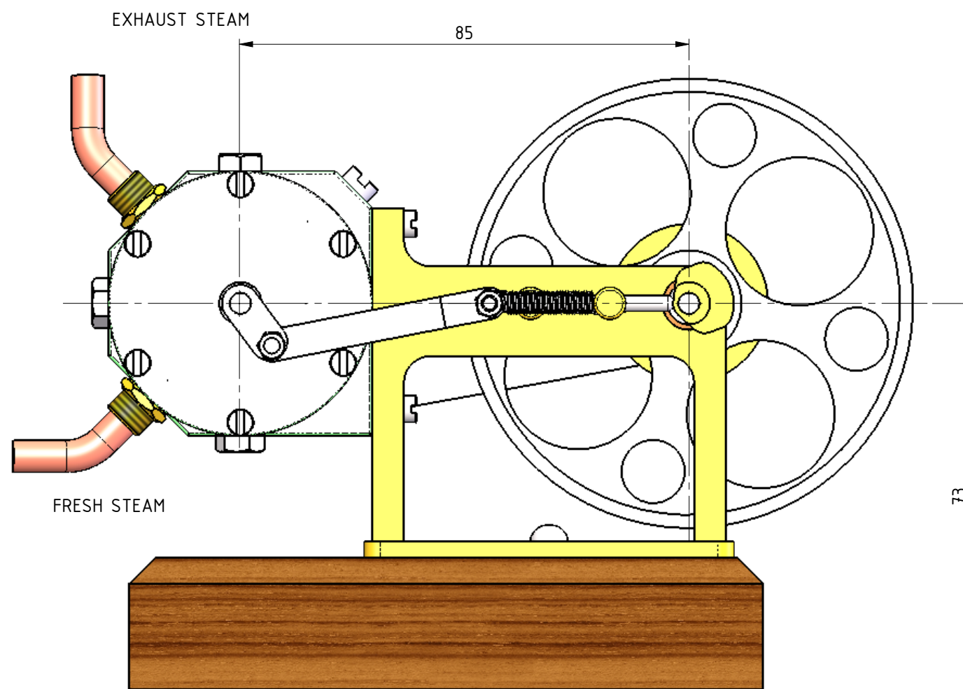
SIDE VIEW
