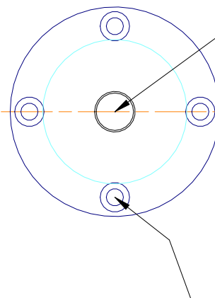
Drill 7.1 thru, tap 9/32 x 32 TPI
