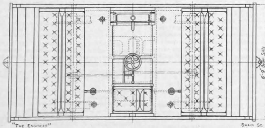
PETROL RAILWAY INSPECTION CAR
