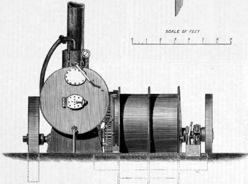
ELEVATION AT FIRE BOX END
