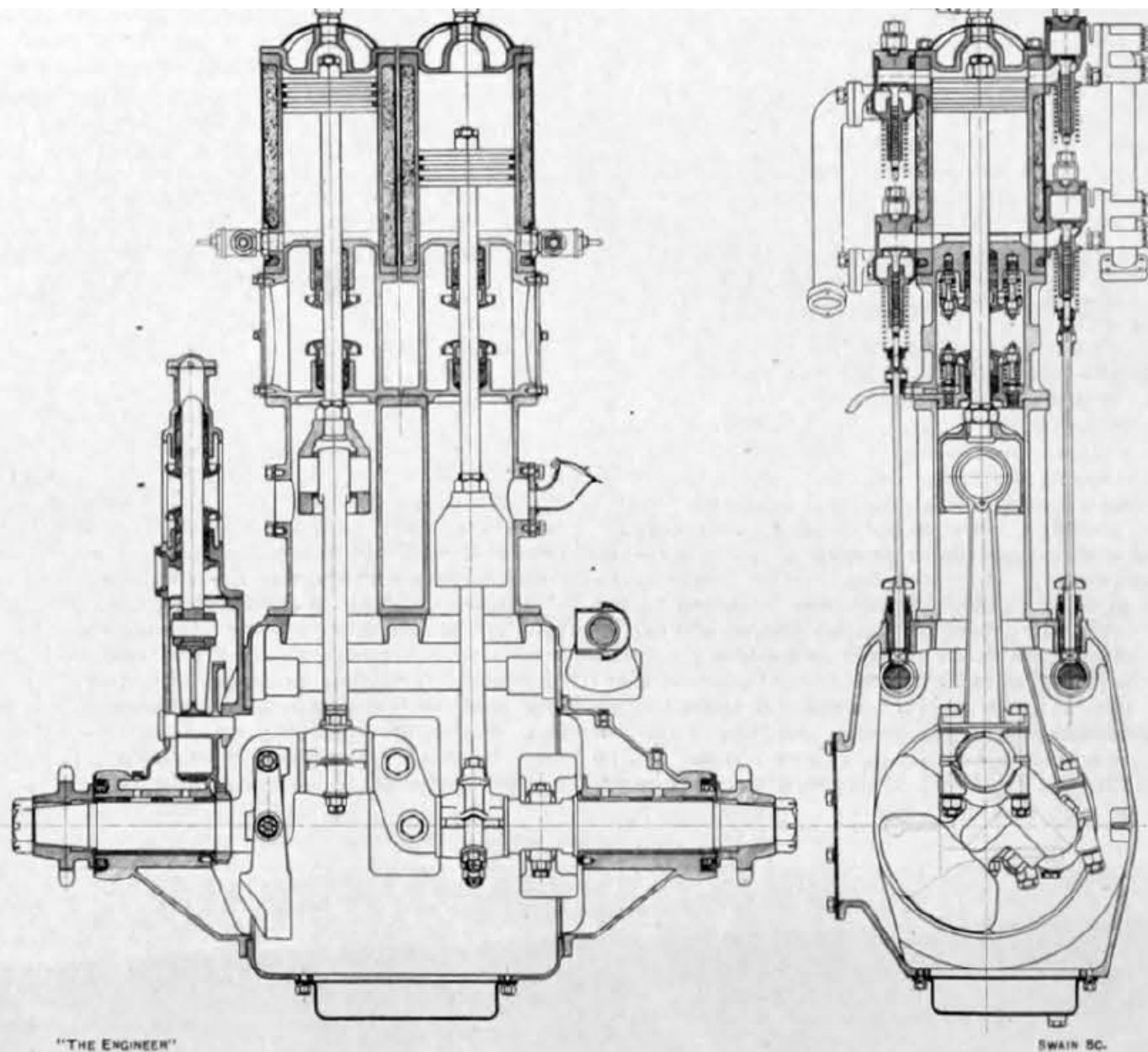
FIG. 2—LONGITUDINAL AND CROSS SECTIONS OF ENGINE
