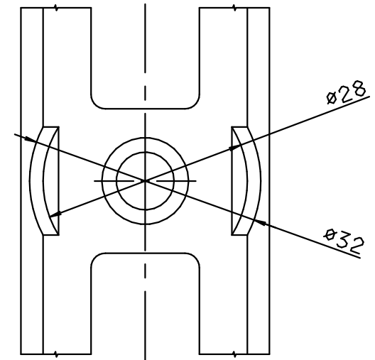
View X
