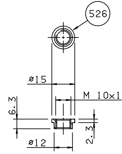
Regulating Valve Bush 1x
