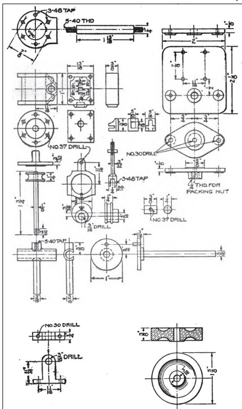
Fig. 95—Detail drawing of the engine
