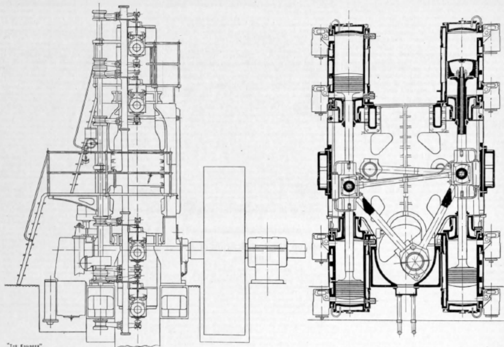
PREMIER SINGLE-CRANK FOUR-CYLINDER VERTICAL GAS ENGINE
