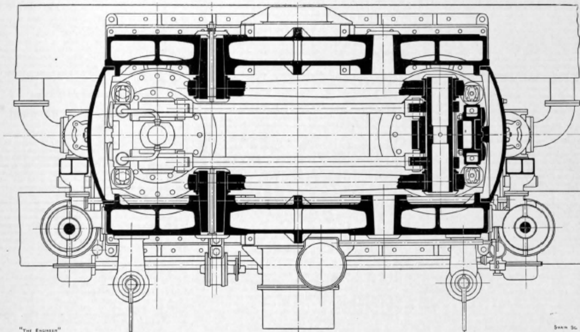
PREMIER VERTICAL GAS ENGINE—HORIZONTAL SECTION
