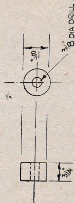
(4) Bolster pad, 1 1/8 in. diameter Br. M.S.
