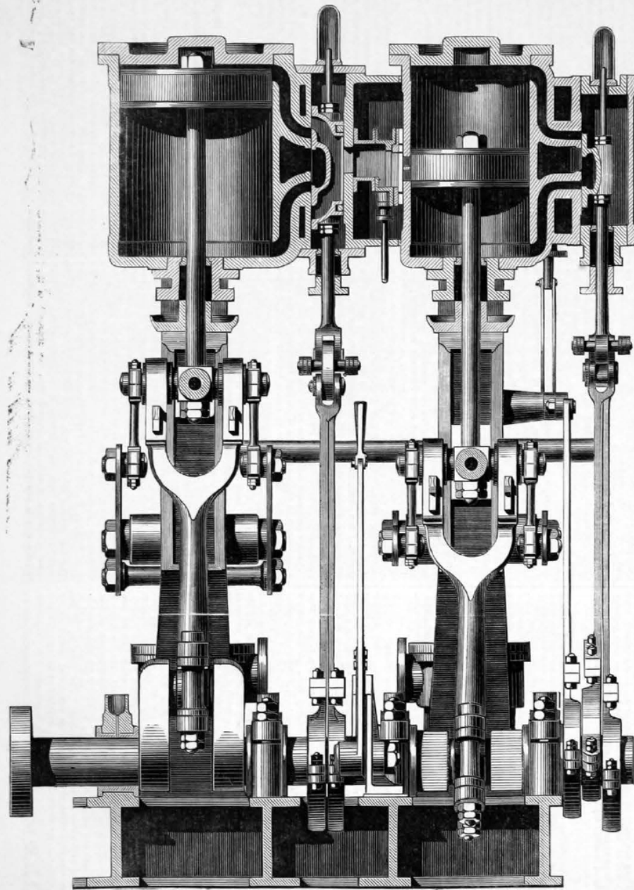
SECTIONAL ELEVATION
