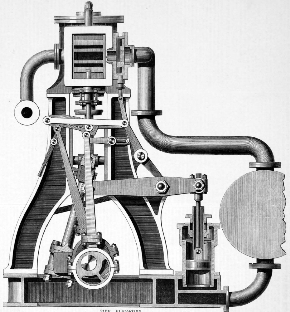
SIDE ELEVATION.
