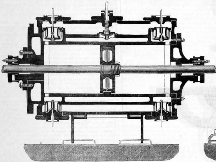
LONGITUDINAL SECTION THRO. CYLINDER & VALVES
