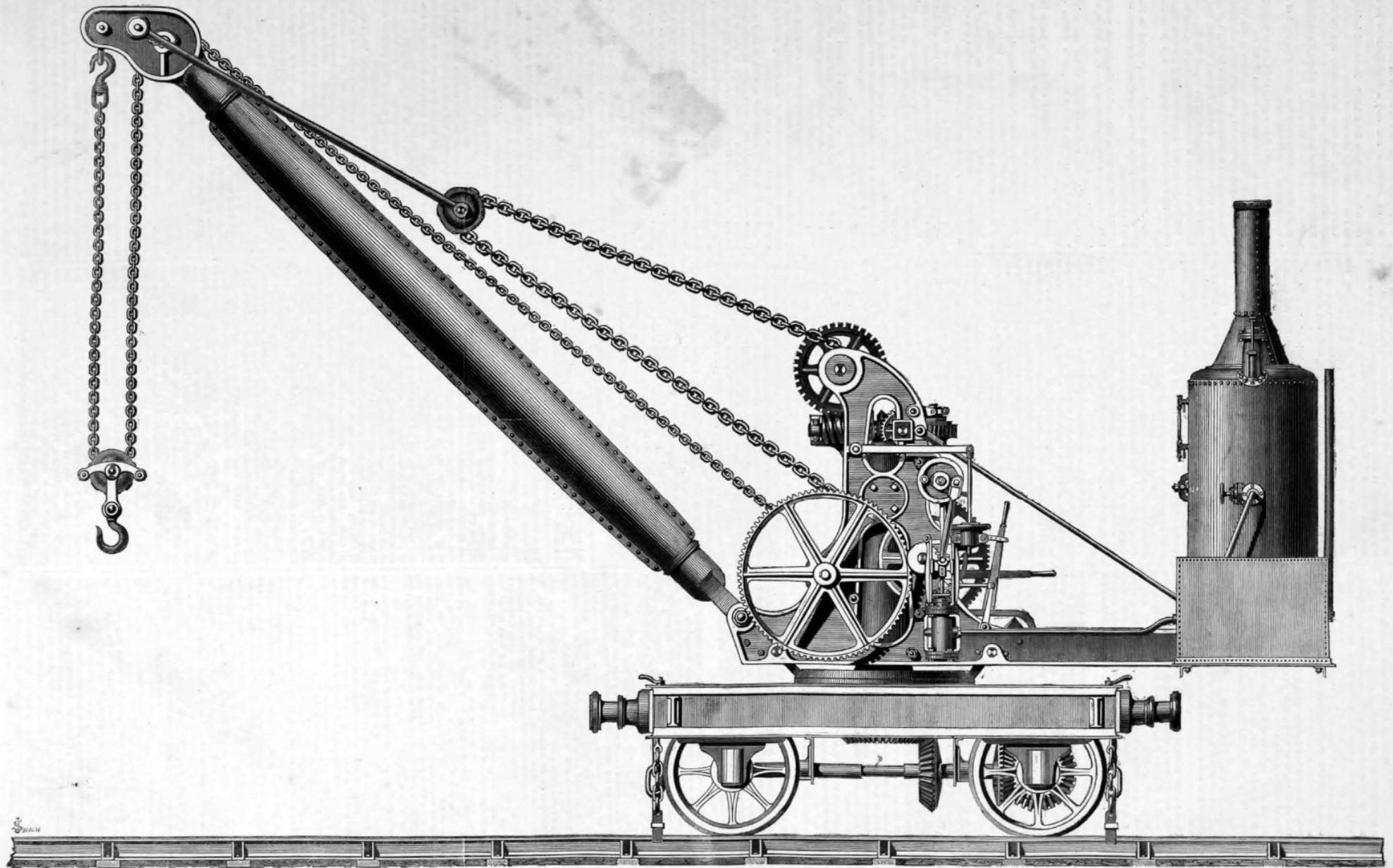
10-TON STEAM TRAVELLING CRANE USED IN THE CONSTRUCTION OF ARMOUR-PLATED VESSELS. CONSTRUCTED BY THE KIRKSTALL FORGE COMPANY.
