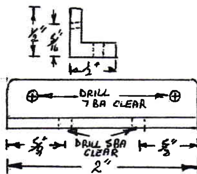
SUPPORT FRAME BRACKETS 2 OFF \frac{1}{2} " x \frac{1}{2} " x \frac{1}{8} " STEEL ANGLE
