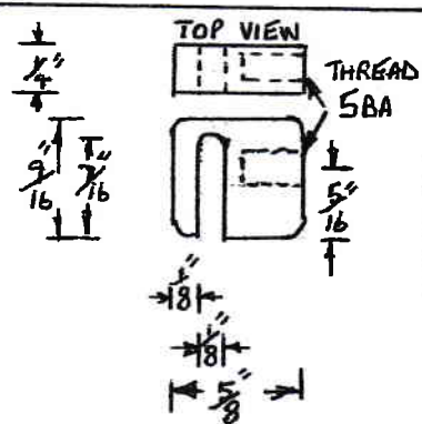
VALVE ROD END 1 OFF BRASS
