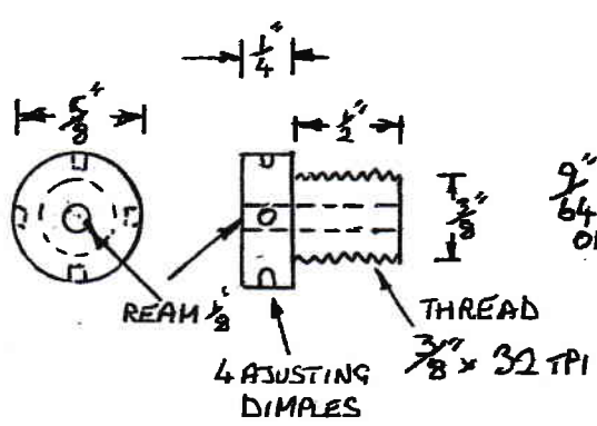
VALVE ROD GLAND 1 OFF BRASS
