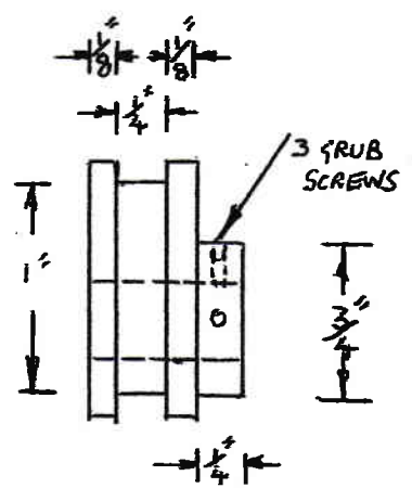
ECCENTRIC SHEAVE 1 OFF CAST IRON OR STEEL
