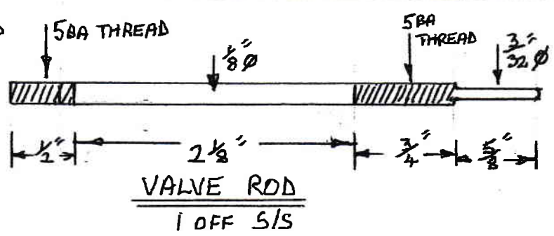
DRAWING TO SHOW OPERATION OF VALVE ROD
