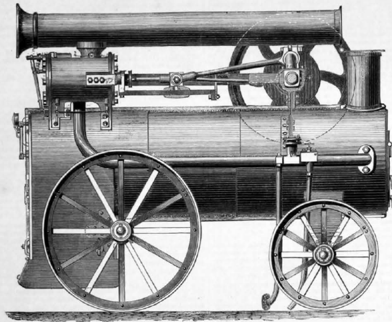
SIDE ELEVATION PLAN
