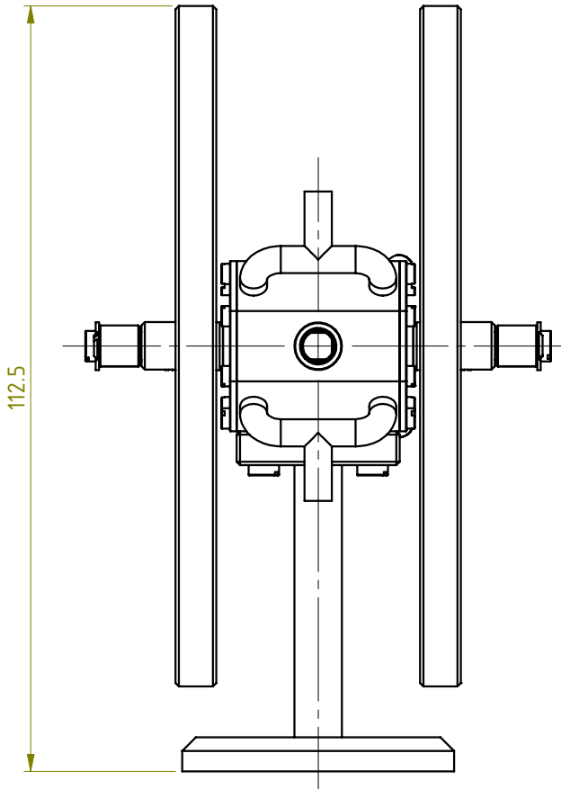
TITLE SINGLE CYLINDER STEAM ENGINE WITH TURNING VALVE GENERAL ARRANGEMENT
